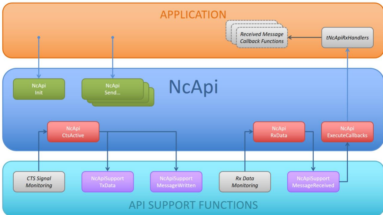
Figure 2 - NcApi structure
